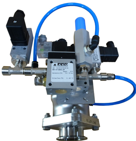
Figure: Pinch valve with a pressure switch → AKOVAC Basic → Safety arrangement (protection circuit) → Pressure switch
